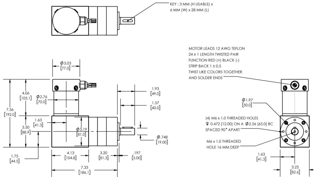
DIMENSIONS ARE INCHES [MM] UNLESS OTHERWISE STATED
